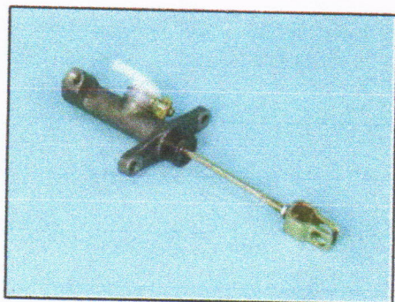
Secondary Clutch Master Assy (Jac Truck)
